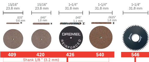
Cut-Off Wheels
